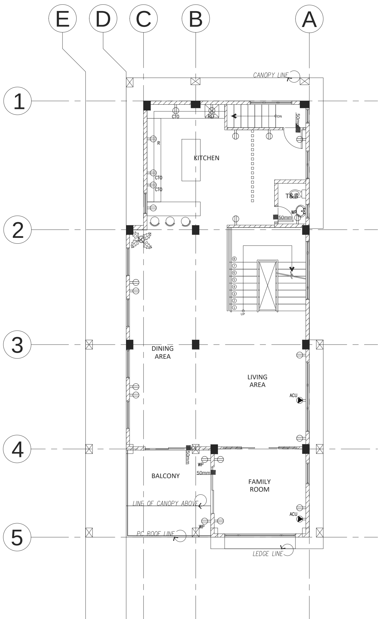
ARANETA RESIDENCE 2 A-00 SECOND POWER LAYOUT SCALE: 1:100 MTS.
