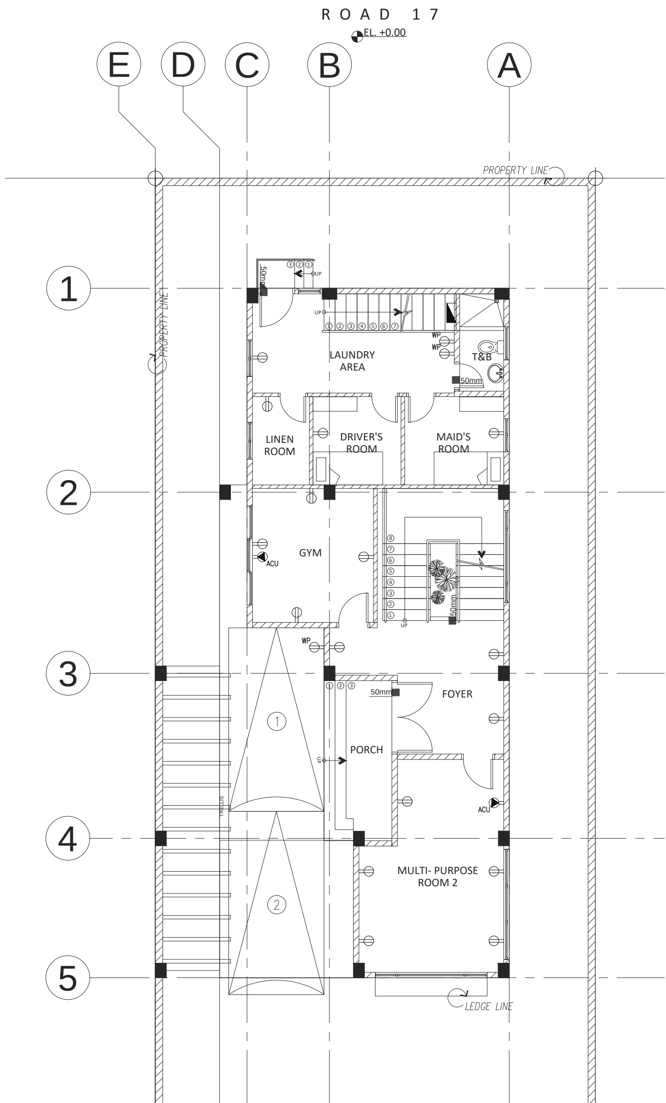
ARANETA RESIDENCE 1 A-00 GROUND POWER LAYOUT SCALE: 1:100 MTS.
